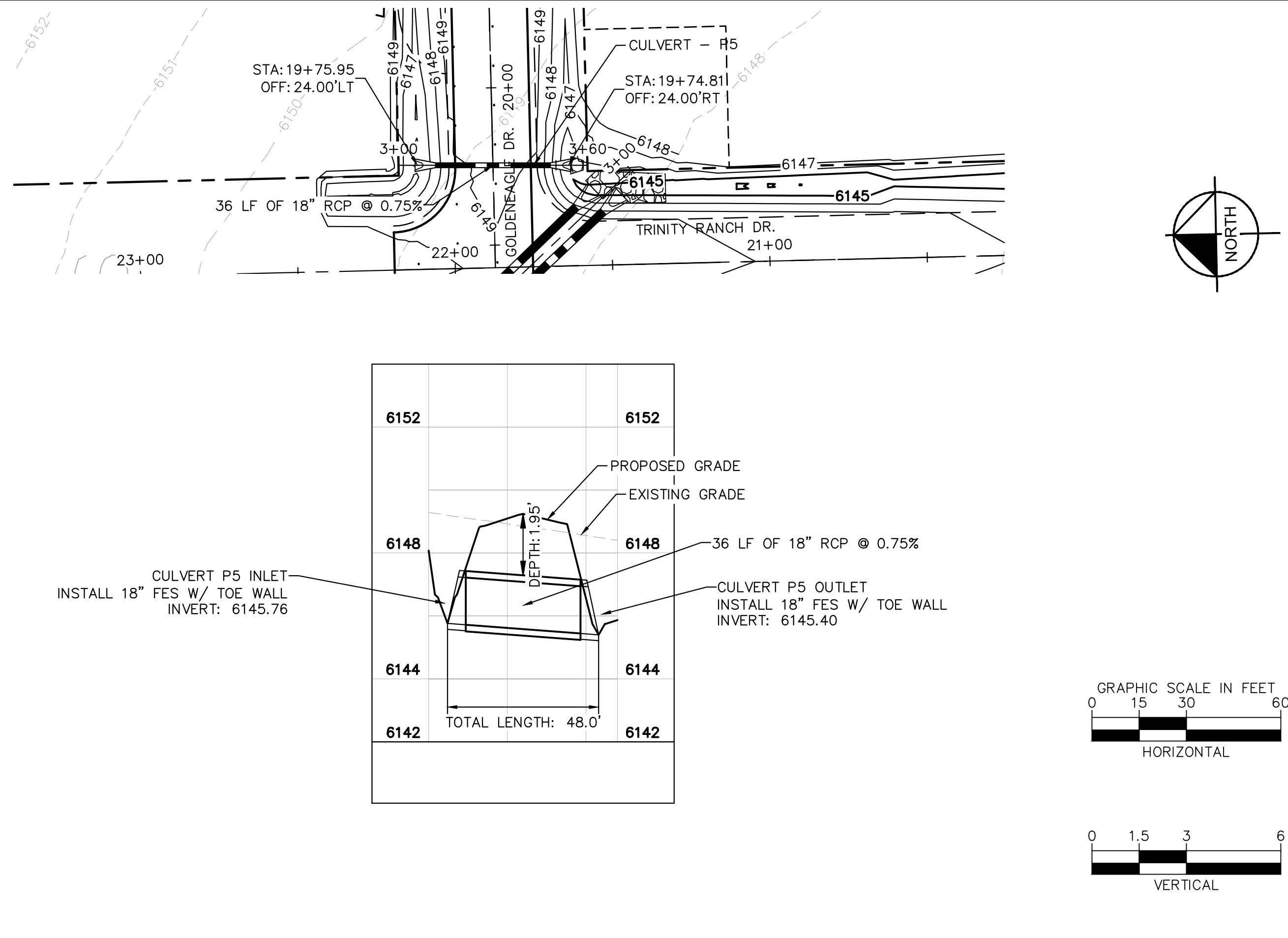
CULVERT P5 PLAN AND PROFILE
