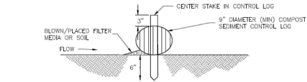
SECTION A COMPOST SEDIMENT CONTROL LOG
