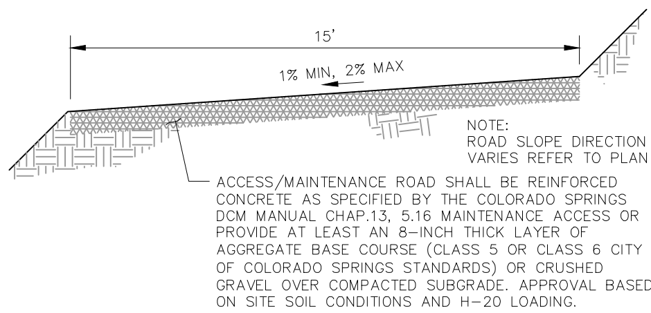
MAINTENANCE & ACCESS ROAD ABOVE EURV TYPICAL SECTION NOT TO SCALE
