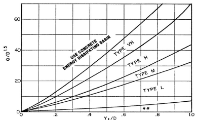
Use D 50 instead of D whenever flow is supercritical in the barrel. ** Use Type L for a distance of 3D downstream.
