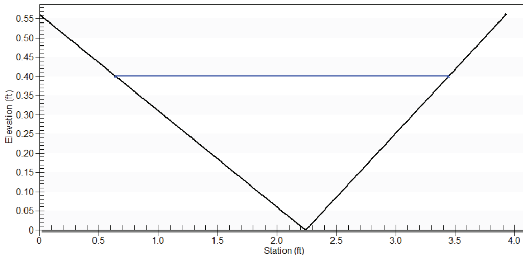
Triangular Channel
