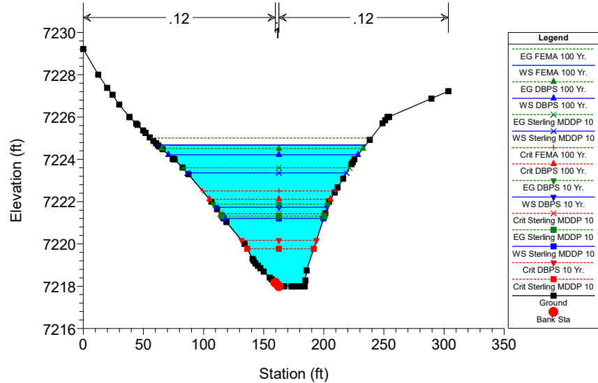
TIMBERRIDGE EXIST. Plan: SC EX 7/24/2019 River = Sand Creek Ex Reach = TimberRidge RS = 4712.26
