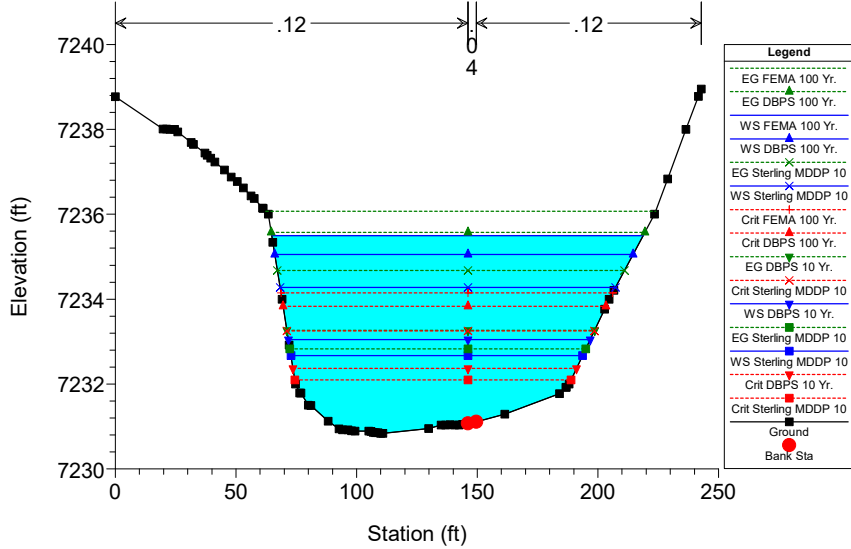
TIMBERRIDGE EXIST. Plan: SC EX 7/24/2019 River = Sand Creek Ex Reach = TimberRidge RS = 4903.69
