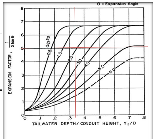
Figure 9-35. Expansion factor for circular conduits
