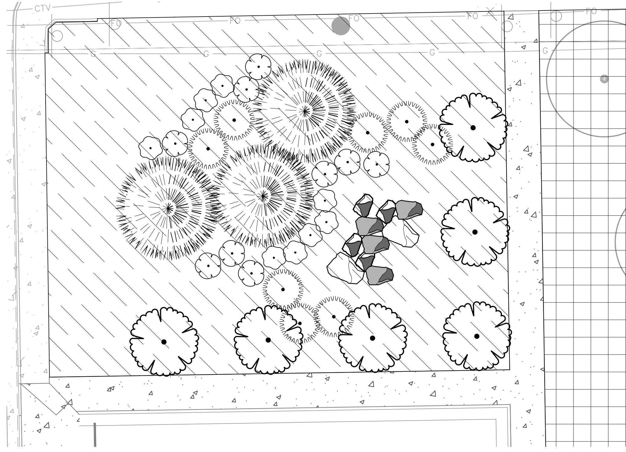
1 XERIC PLANTING ENLARGEMENT L1.0 PLAN 1" = 10'-0"
