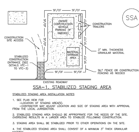
Stabilized Staging Area (SSA) SM-6
