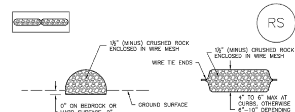
ROCK SOCK SECTION
