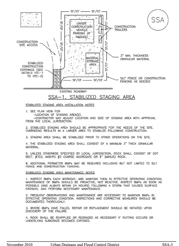
SSA-3 Urban Drainage and Flood Control District November 2010 Urban Storm Drainage Criteria Manual Volume 3
