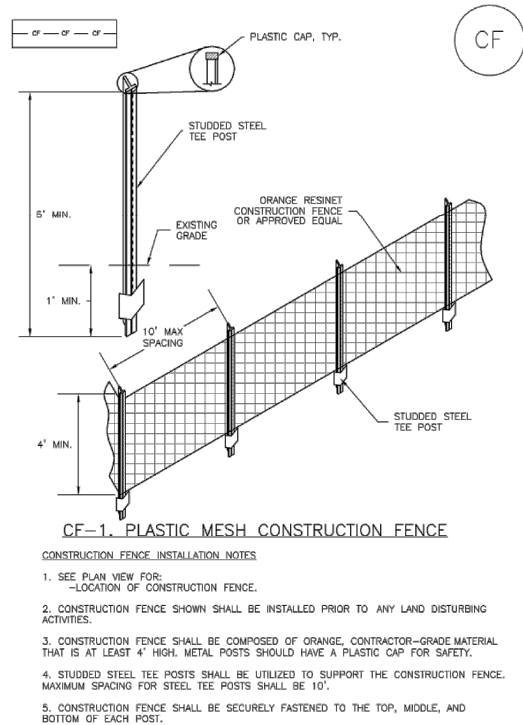
CF-2 Urban Drainage and Flood Control District November 2010 Urban Storm Drainage Criteria Manual Volume 3
