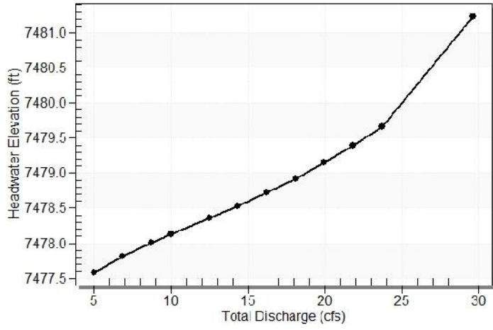
Total Rating Curve Crossing: Crossing B9
