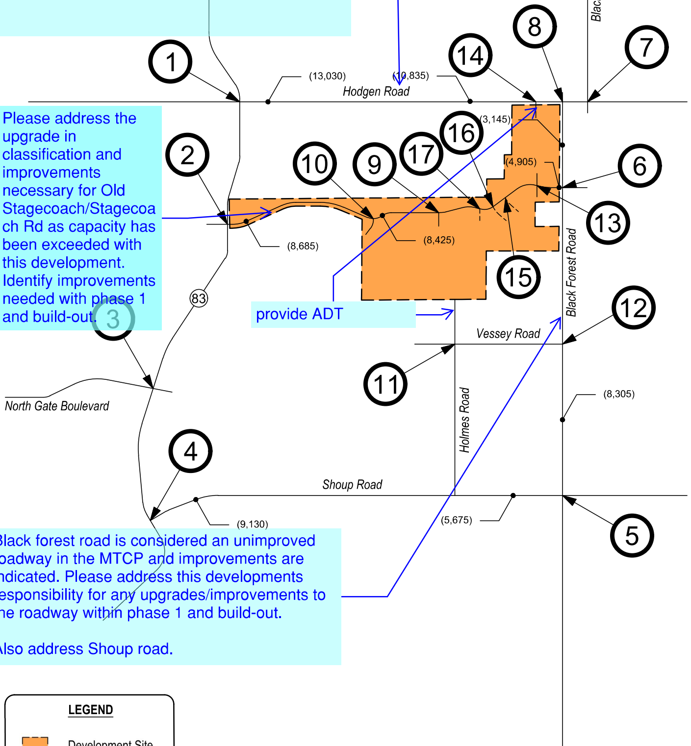
Figure 16 TOTAL TRAFFIC - YEAR 2027 Volumes (ADT) : Average Daily Traffic
