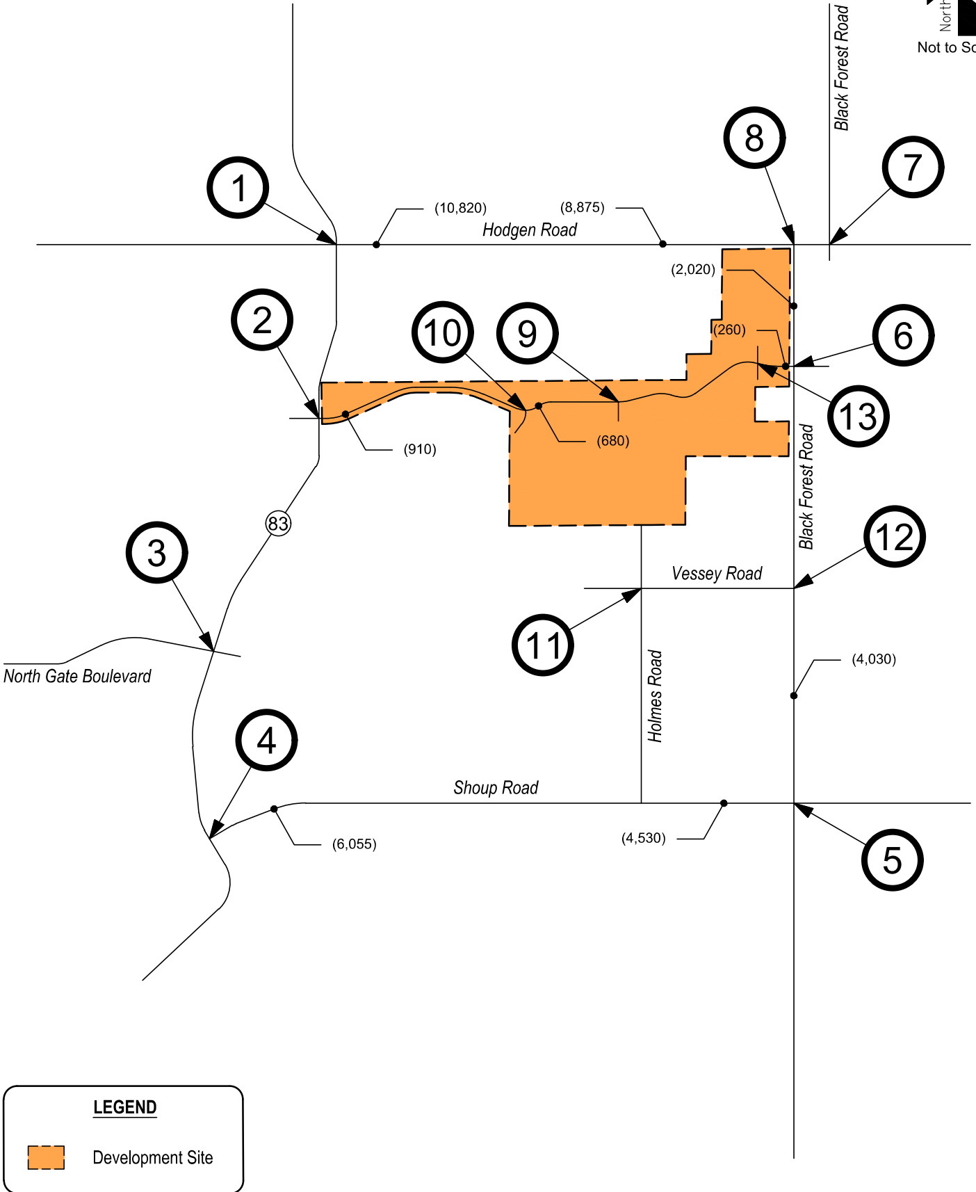
Figure 3 EXISTING TRAFFIC Volumes (ADT) : Average Daily Traffic
