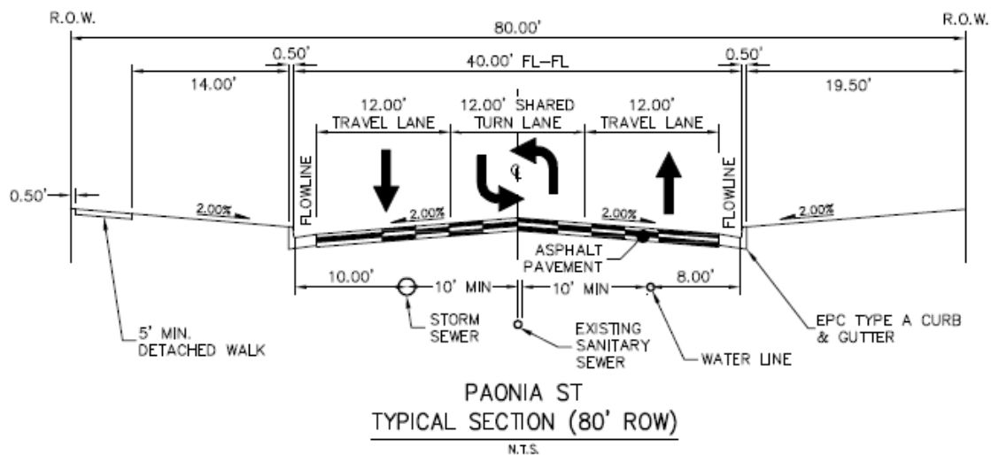
Figure 10. Proposed Paonia Street Cross Section
