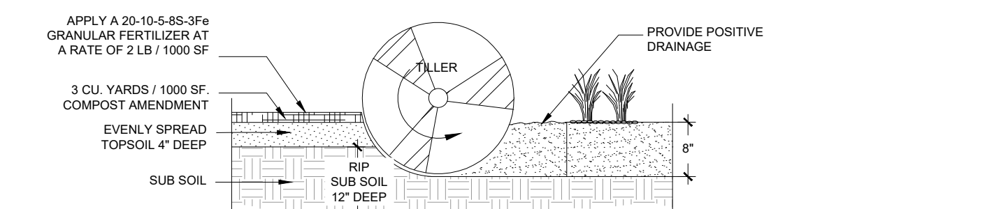
3 L1 SOIL PREP- SEED AREAS PLANTING DETAIL NTS
