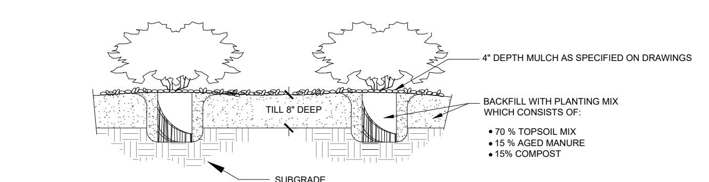
5 L1 SHRUB DETAIL PLANTING DETAIL NTS
