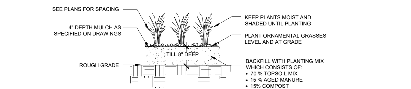
6 L1 GRASS & PERENNIAL DETAIL PLANTING DETAIL NTS
