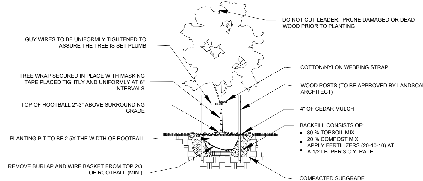
2 L1 DECIDUOUS TREE PLANTING DETAIL NTS
