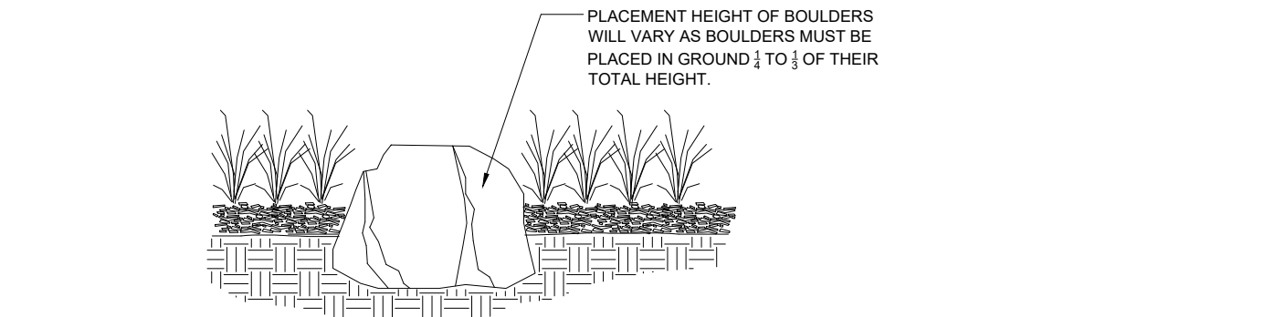
4 L1 BOULDER DETAIL NTS
