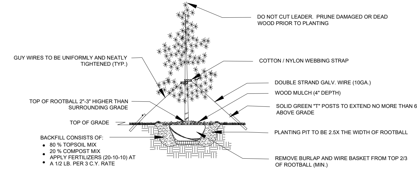
1 L1 EVERGREEN TREE PLANTING DETAIL NTS
