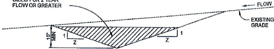
A. EXCAVATED SWALE
