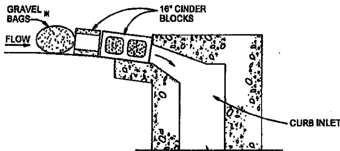
SECTION
