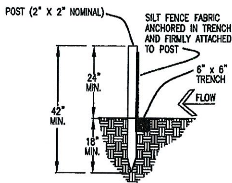
SILT FENCE
