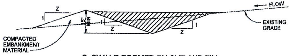
C. SWALE FORMED BY CUT AND FILL
