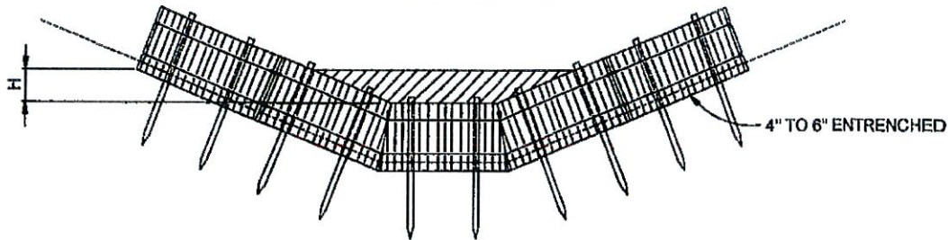
B. STRAW BALE CHECK DAM
