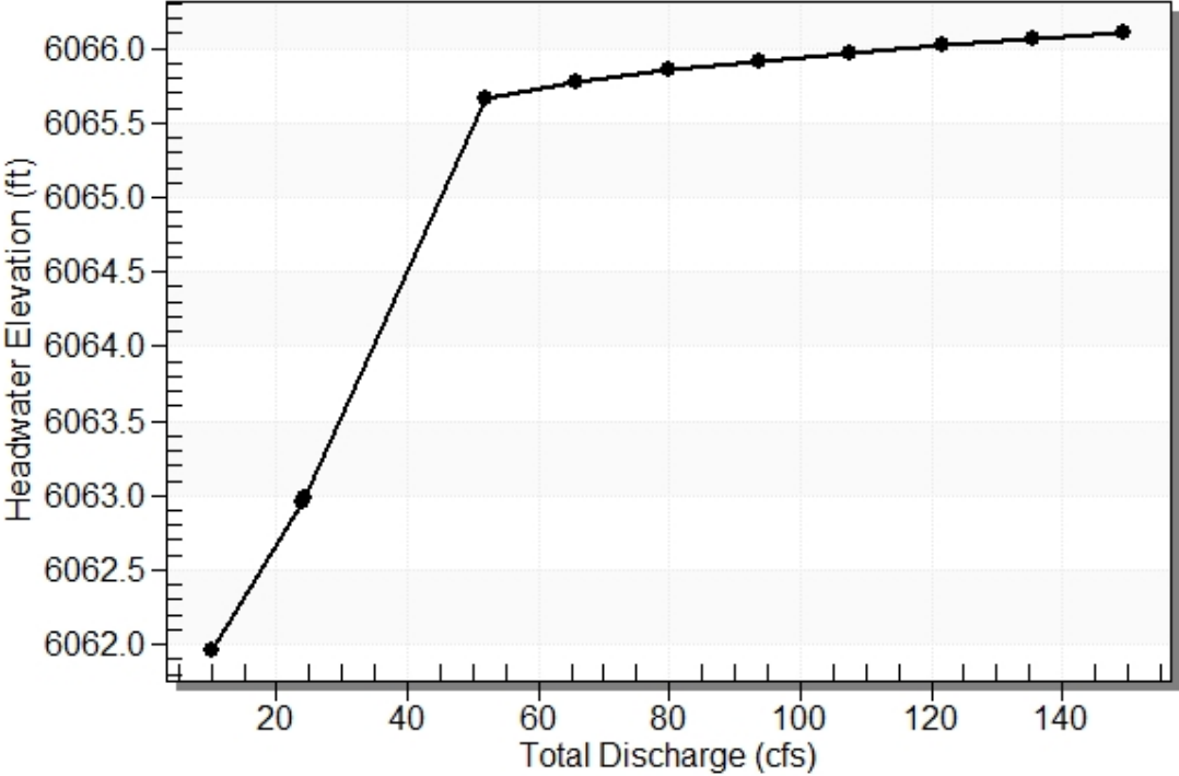
Total Rating Curve Crossing: Crossing EC11
