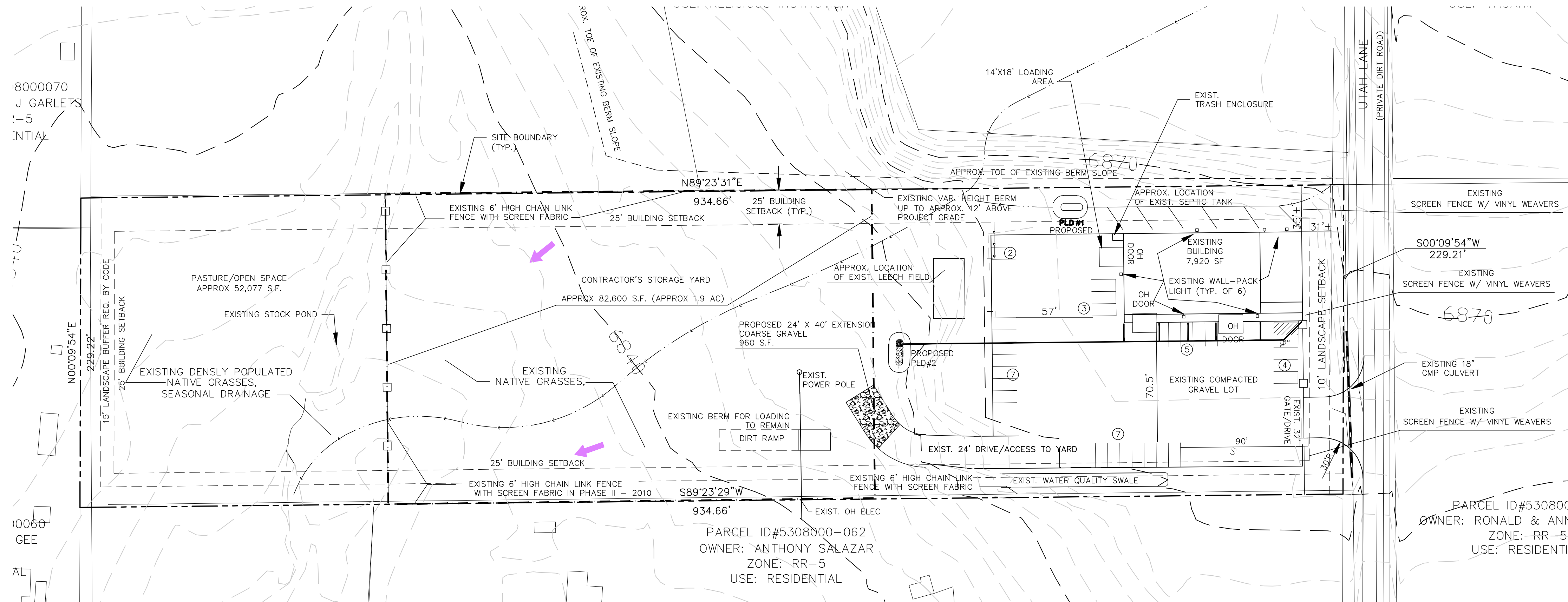
SITE PLAN 1"=50'
