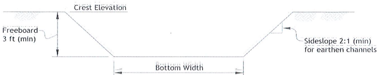
Spillway Section
