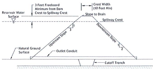
Cross Section Through Dam at Outlet
