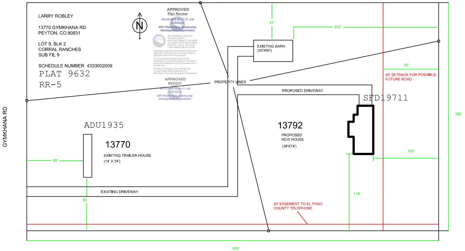
PLOT PLAN
