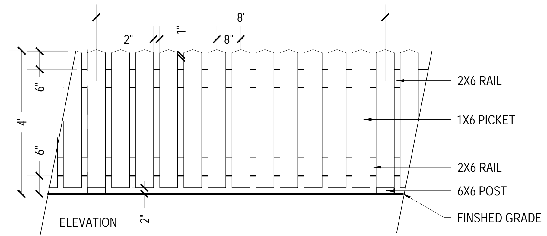
7 4' FENCE FOR FRONT LOADED LOTS NTS
