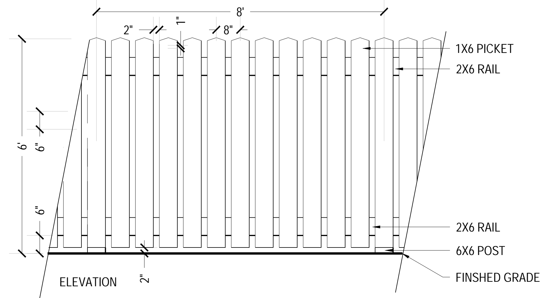
8 6' FENCE FOR REAR LOADED LOTS NTS
