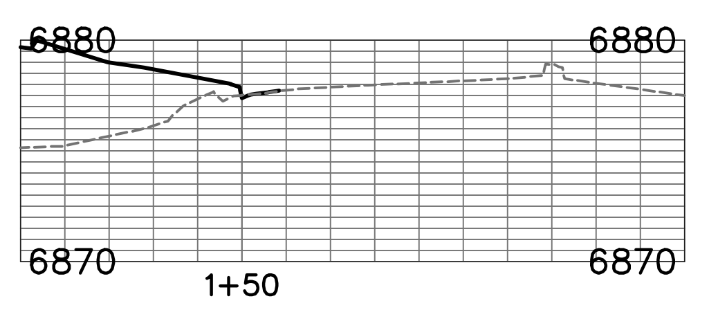
MERIDIAN ROAD X-SECTIONS
