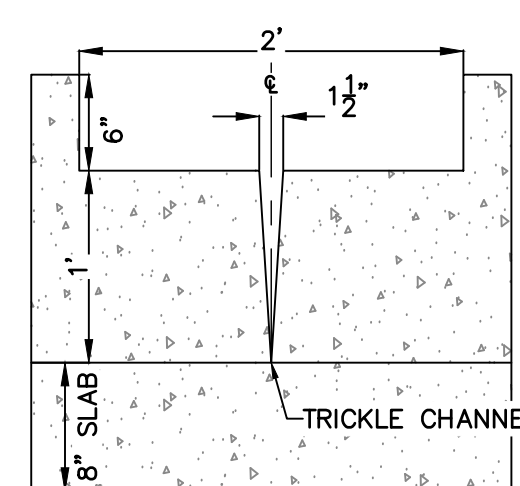
FOREBAY B1 & B2 WALL SECTION
