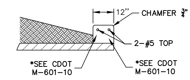
RCP HEADWALL
