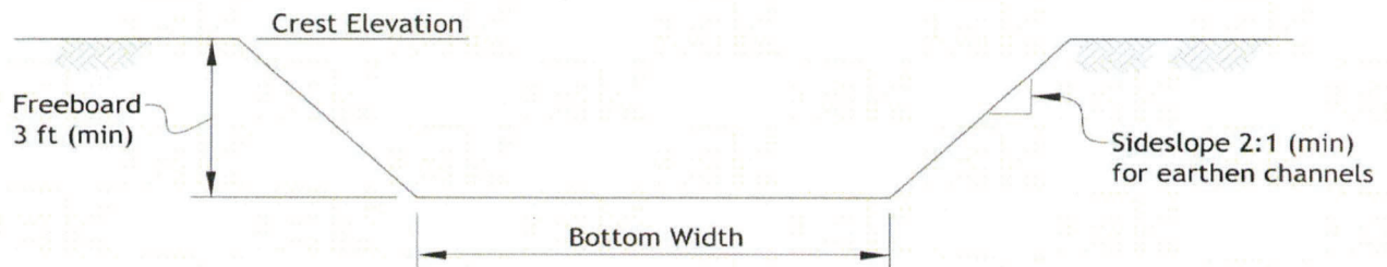
Spillway Section
