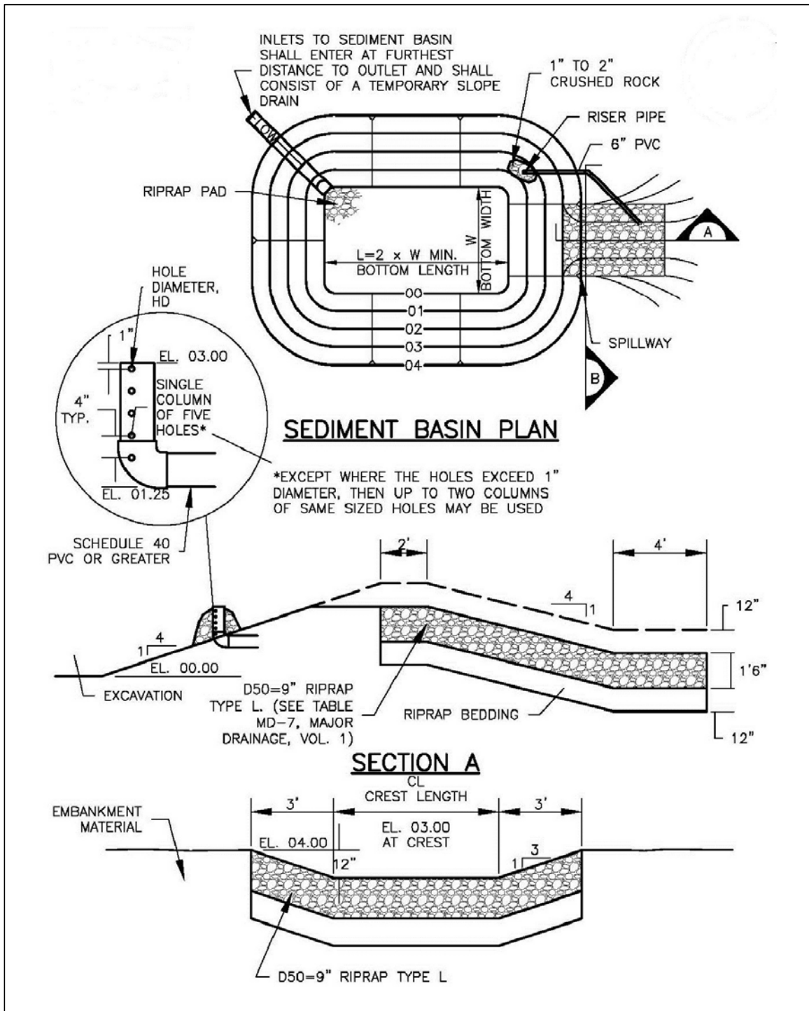
TEMPORARY SEDIMENT BASIN
