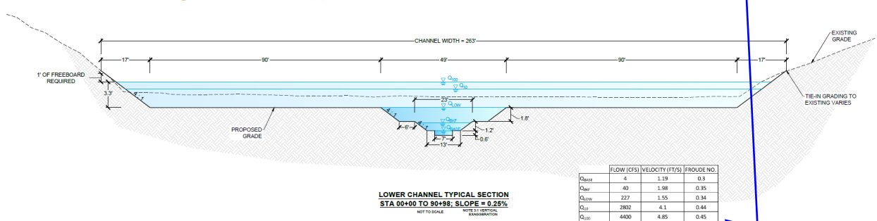
Figure 7. Typical Lower Channel Section
