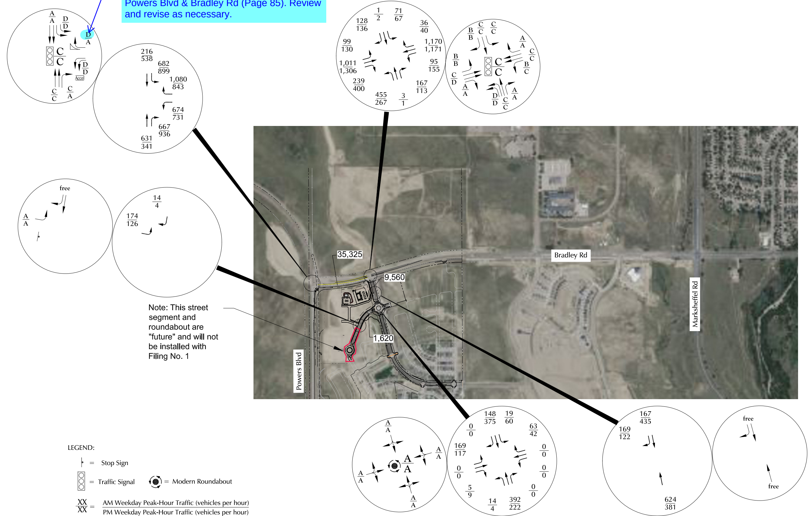
Figure 15 2031 Total Traffic, Lane Geometry, Traffic Control, and Level of Service Waterview East Commercial Filing No. 1 (LSC #S214971)
