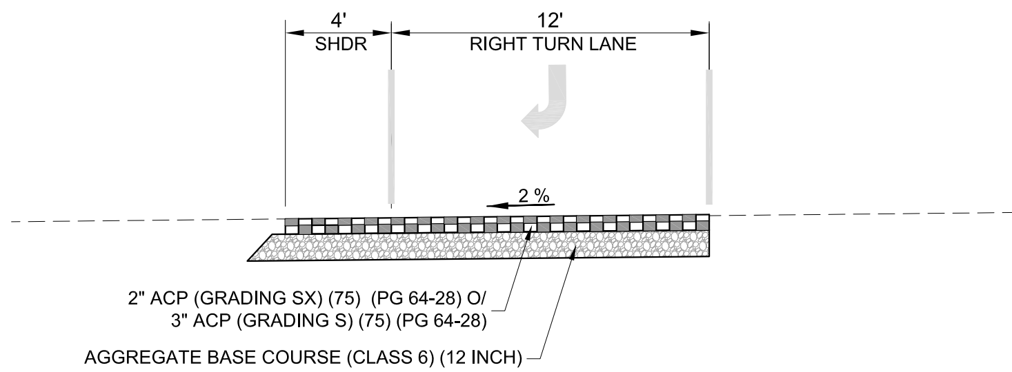
STRUCTURE SECTION
