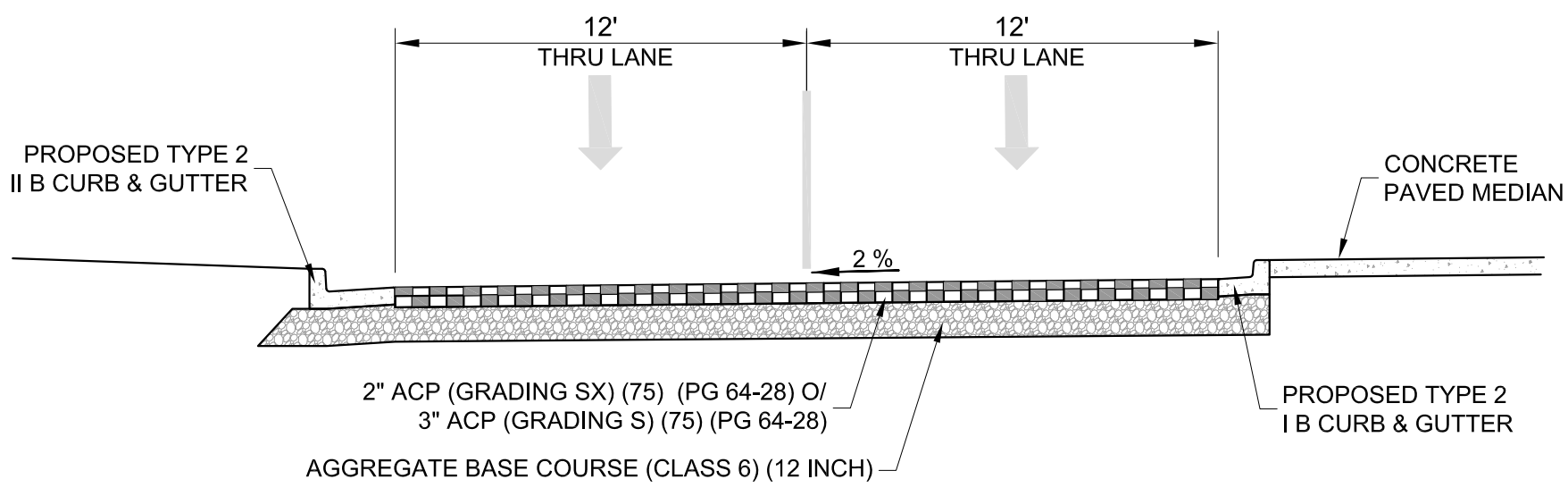
STRUCTURE SECTION
