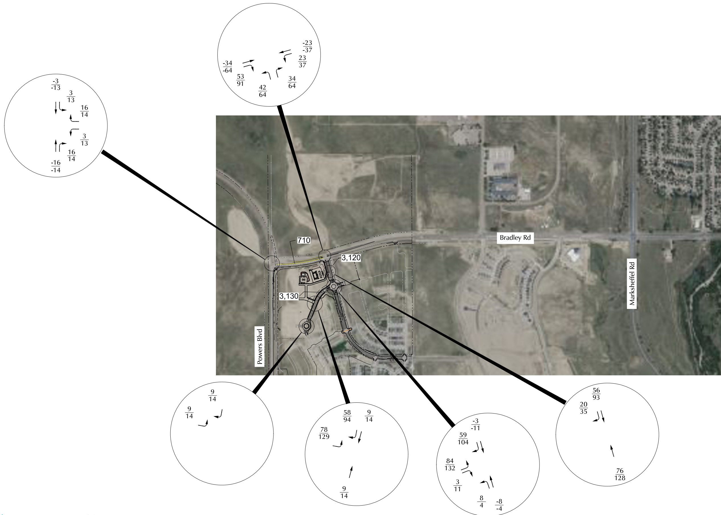
Figure 10b Pass-by Future Waterview East Commercial Filings-Generated Traffic Waterview East Commercial Filing No. 1 (LSC #S214971)
