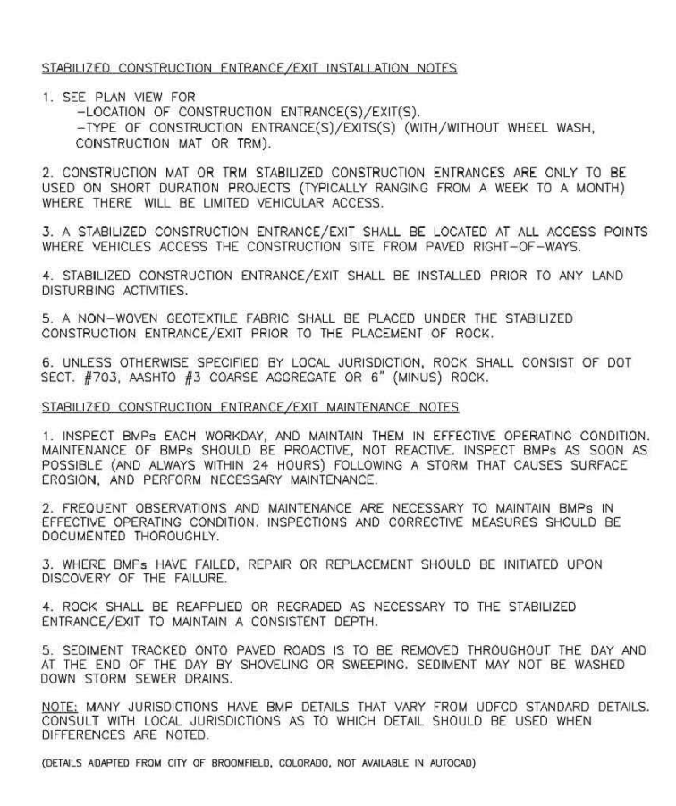
SM-4. STABILIZED CONSTRUCTION ENTRANCE/EXIT INSTALLATION NOTES
