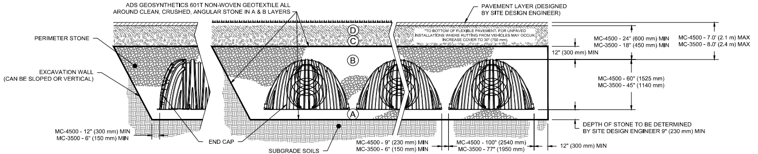
Figure 2 - Fill Material Locations
