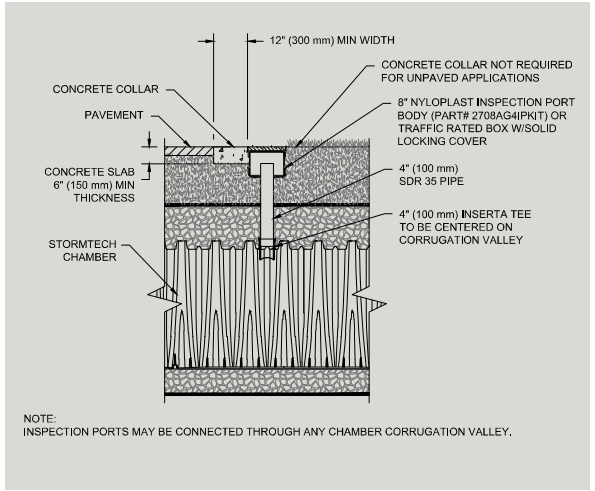
Figure 1- Inspection Port Detail
