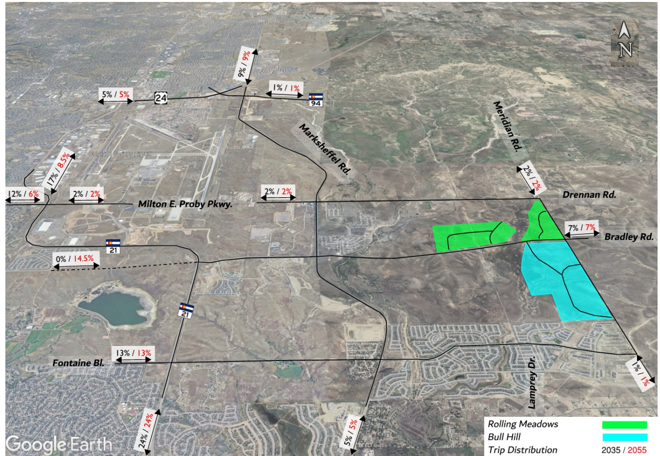
Figure 10. Trip Distribution
