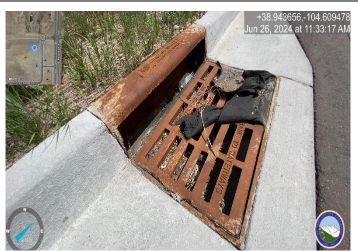
Photo 2: Northern inlets near pond embankment have drop bags installed. Remove and clear debris from inlets.
