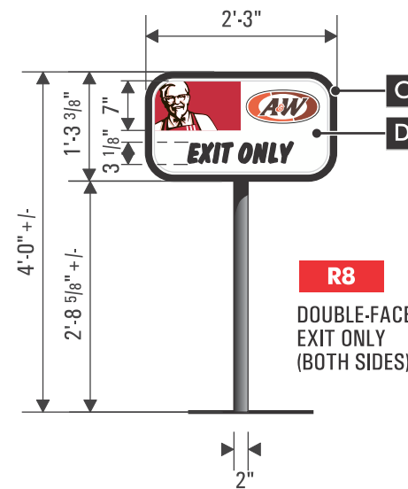
R8 R9 D/F DIRECTIONAL (ILLUMINATED) SCALE: 3/8" = 1'-0" QUANTITY: (2 EA) RECEIVE & INSTALL (NEW FOUNDATION REQUIRED. CUT EXCESS PIPE TO COMPLY WITH CODE)
