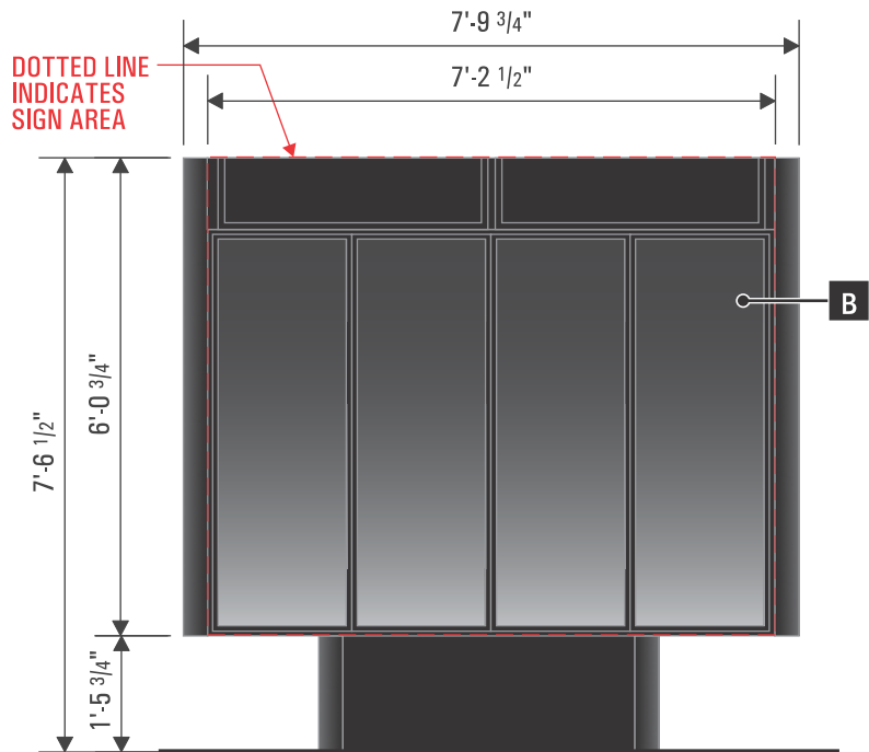
R3 S/F MENU CABINET (ILLUMINATED) SCALE: 3/8" = 1'-0" QUANTITY: 1 RECEIVE & INSTALL (RE-USE EXISTING MATCHPLATE)
