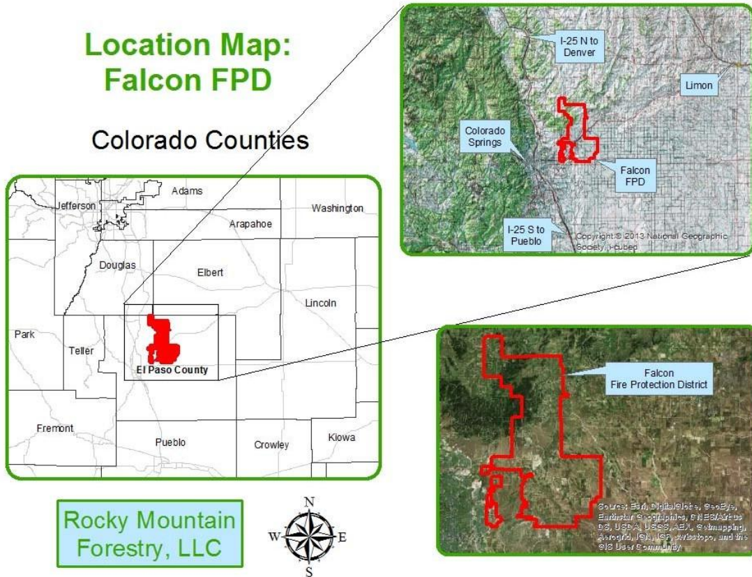
Vicinity Map showing location of FFPD
