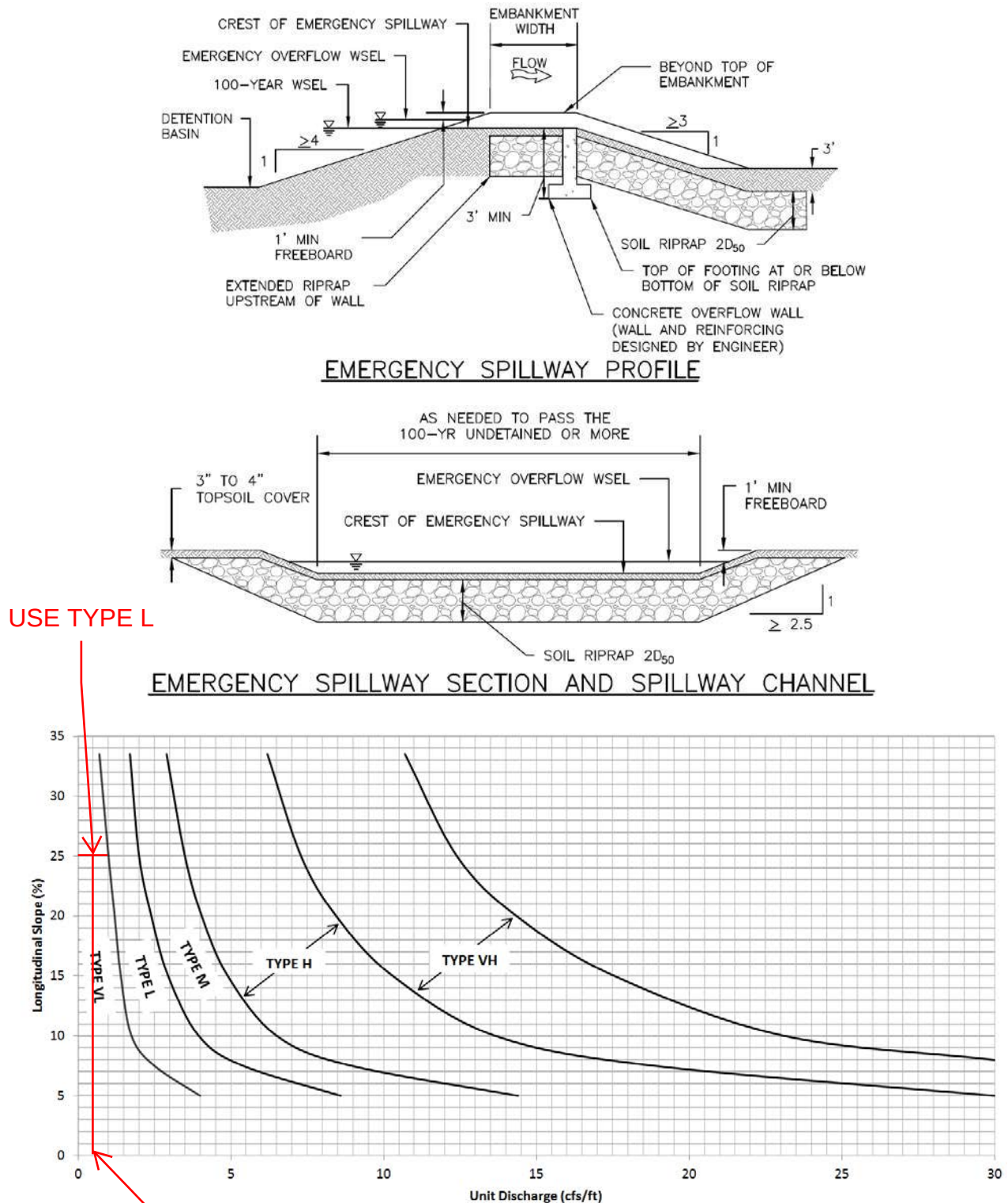
Figure 12-21. Embankment protection details and rock sizing chart (adapted from Arapahoe County)
