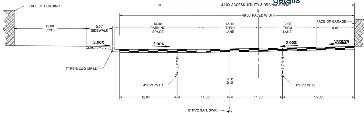
APISHAPA HEIGHTS - W/ GARAGE TYPICAL SECTION - 1 (PRIVATE DRIVE)
