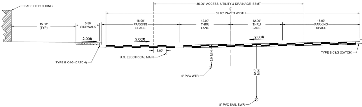
SEGUNDO GROVE TYPICAL SECTION - 4 (PRIVATE LOCAL)
