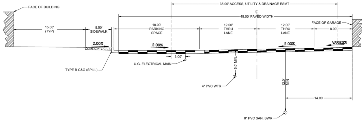
SEGUNDO GROVE - W/ GARAGE TYPICAL SECTION - 3 (PRIVATE DRIVE)
