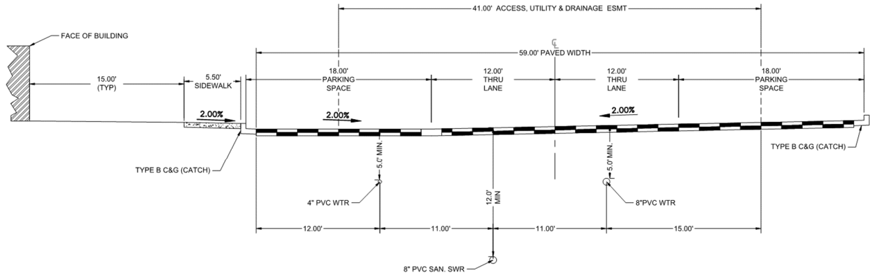
APISHAPA HEIGHTS - TYPICAL SECTION - 2 (PRIVATE DRIVE)
