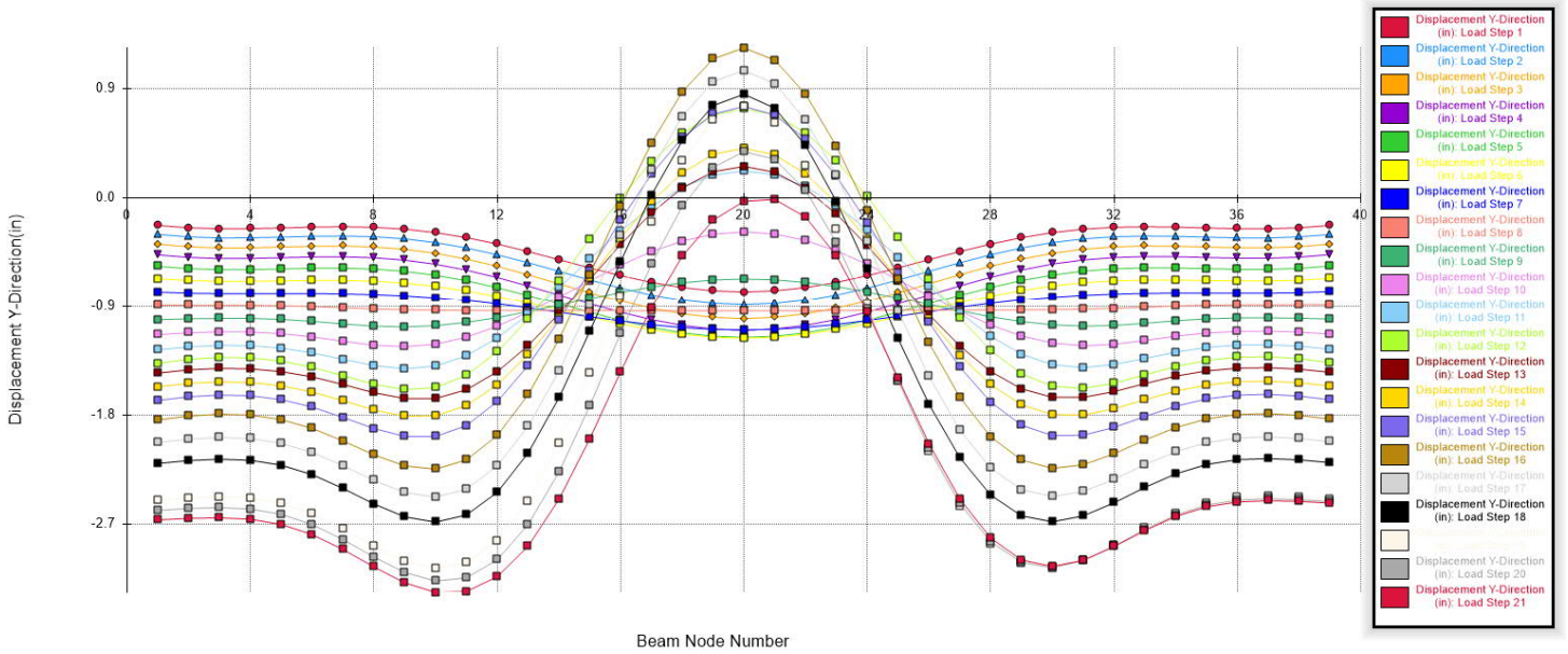
Displacement Y-Direction(in): Load steps 1,2,3,4,5,6,7,8,9,10,11,12,13,14,15,16,17,18,19,20,21,
