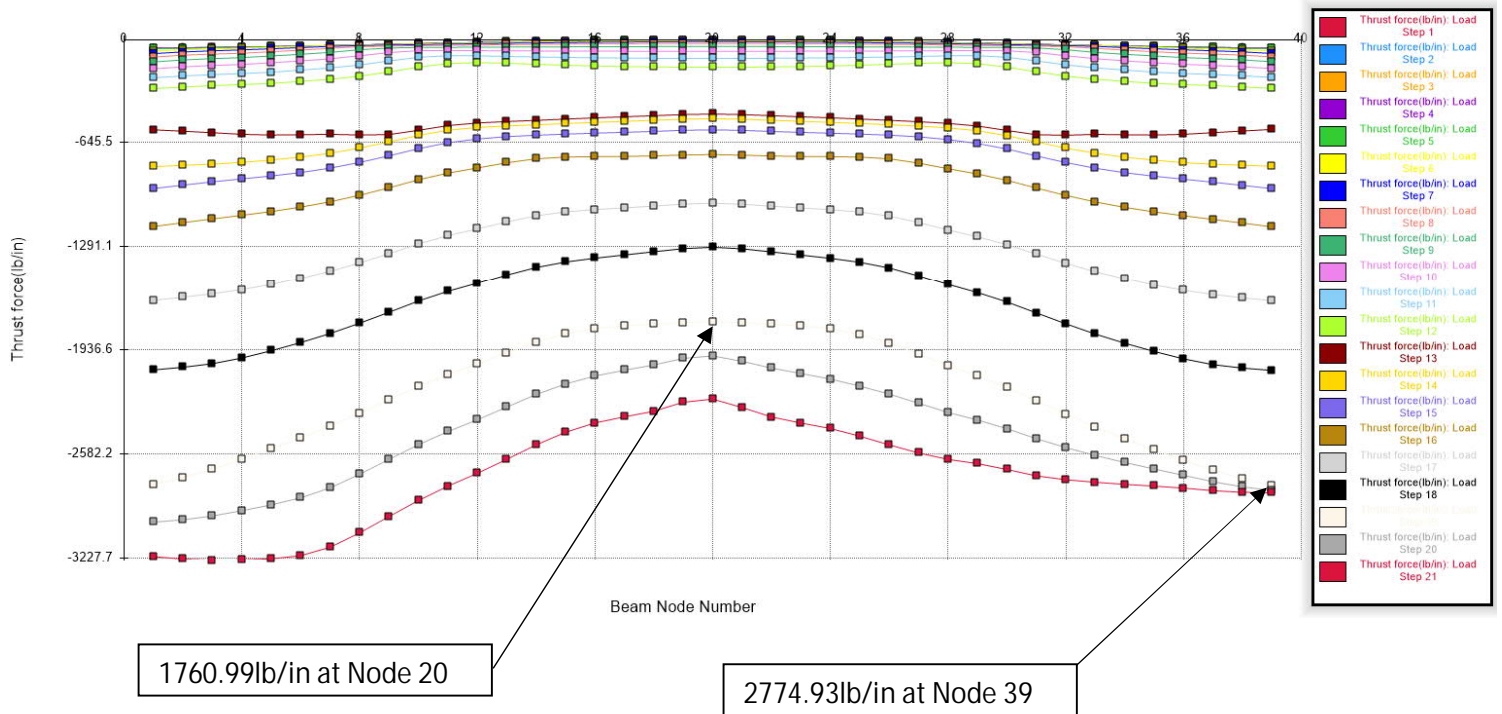
Thrust force(lb/in): Load steps 1,2,3,4,5,6,7,8,9,10,11,12,13,14,15,16,17,18,19,20,21,
