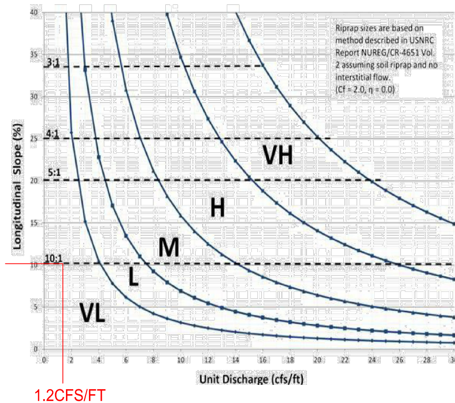
Figure 13-12d. Riprap Types for Emergency Spillway Protection
