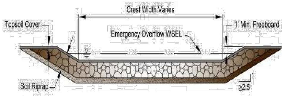
Figure 13-12c. Emergency Spillway Protection
