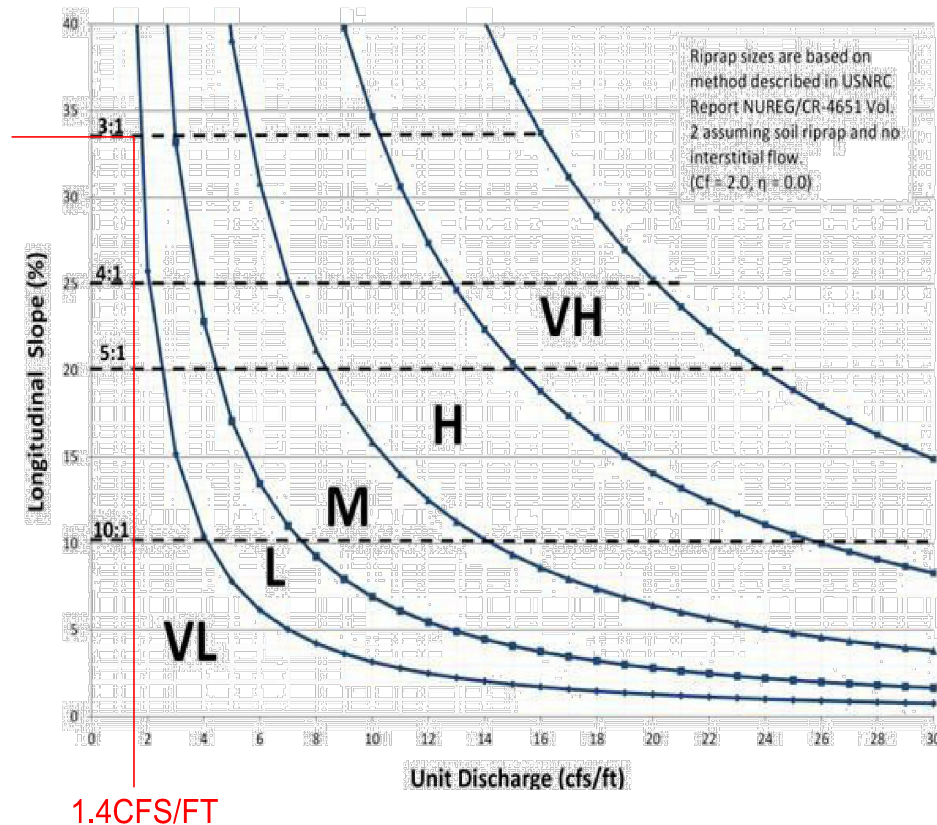
Figure 13-12d. Riprap Types for Emergency Spillway Protection
