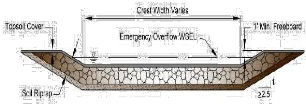
Figure 13-12c. Emergency Spillway Protection
