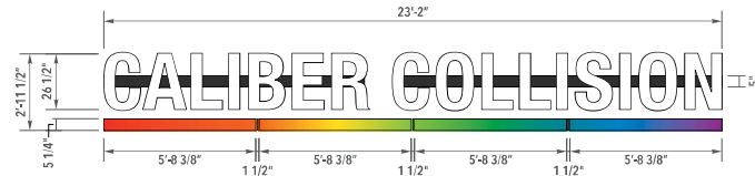
1 RELOCATE EXISTING ILLUMINATED CHANNEL LETTERS - RACEWAY SCALE: 1/4" = 1'-0"
