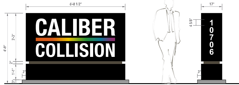
2 D/F ILLUMINATED MONUMENT SIGN SCALE: 1/2" = 1'-0"
