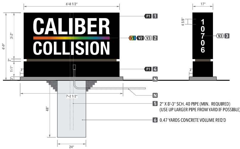
2 D/F ILLUMINATED MONUMENT SIGN SCALE: 1/2" = 1'-0"
