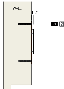
SIDE SECTION DETAIL SCALE: 1 1/2" = 1'-0"
