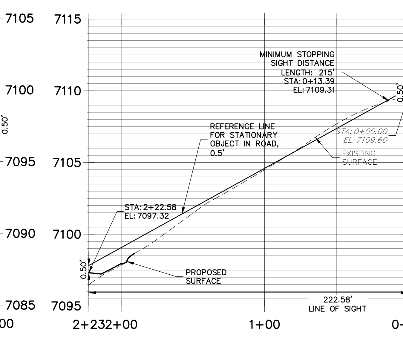
STOPPING SIGHT VIEW CORRIDOR (SOUTH) STA 0+00.00 TO 2+22.58
