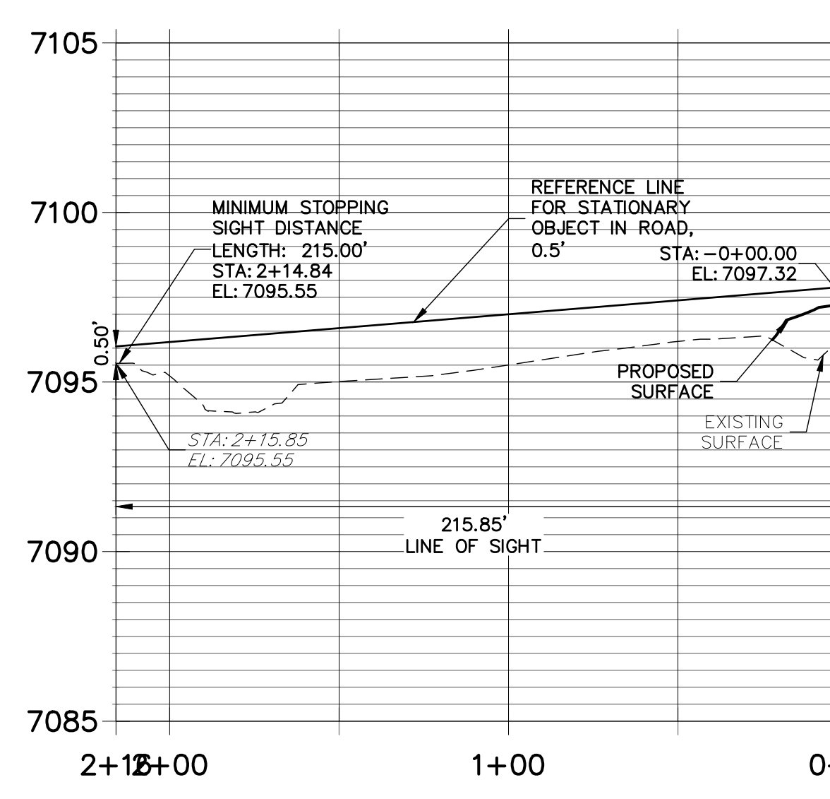
STOPPING SIGHT VIEW CORRIDOR (NORTH) STA 0+00.00 TO 2+15.85
