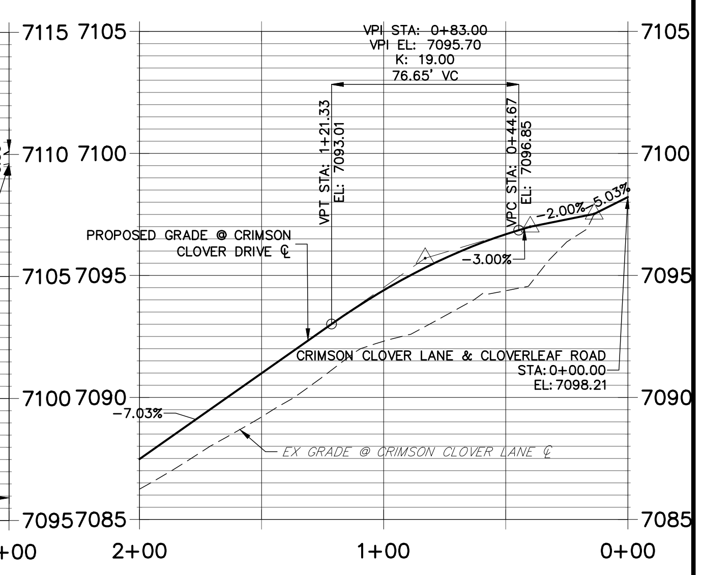
CRIMSON CLOVER DRIVE PROFILE STA 0+00.00 TO 2+00.00
