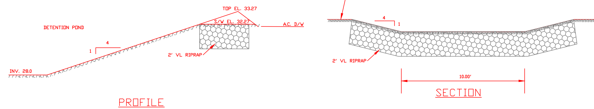
SPILLWAY DETAILS
