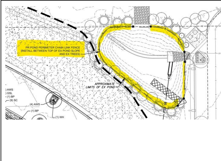
Photo 1: PR Pond perimeter chain link fence (install between top of existing pond slope and existing trees) Verify in As-Builds, Missing fence in field.
