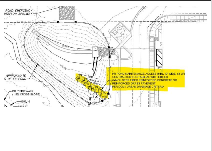
Photo 2: PR Pond maintenance access (min 10' wide, 54 LF) Stabilize with 6" deep fiber reinforced concrete or reinforced grass pavement pe UDC manual.
