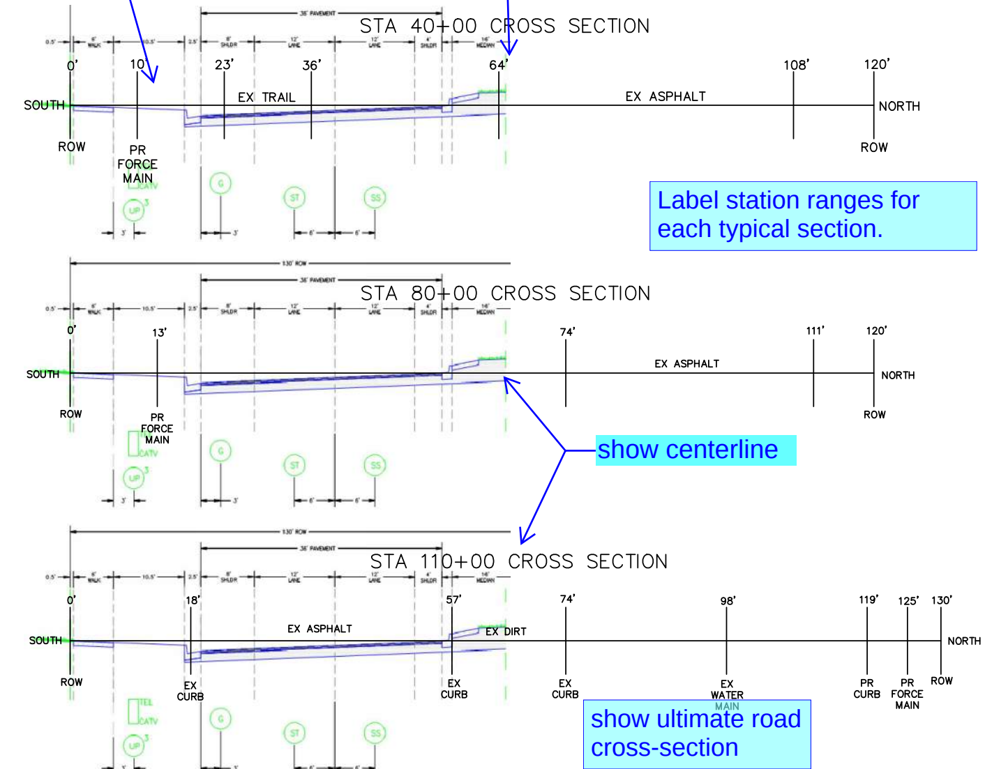
STAPLETON ROW CROSS SECTIONS 1" = 20'
