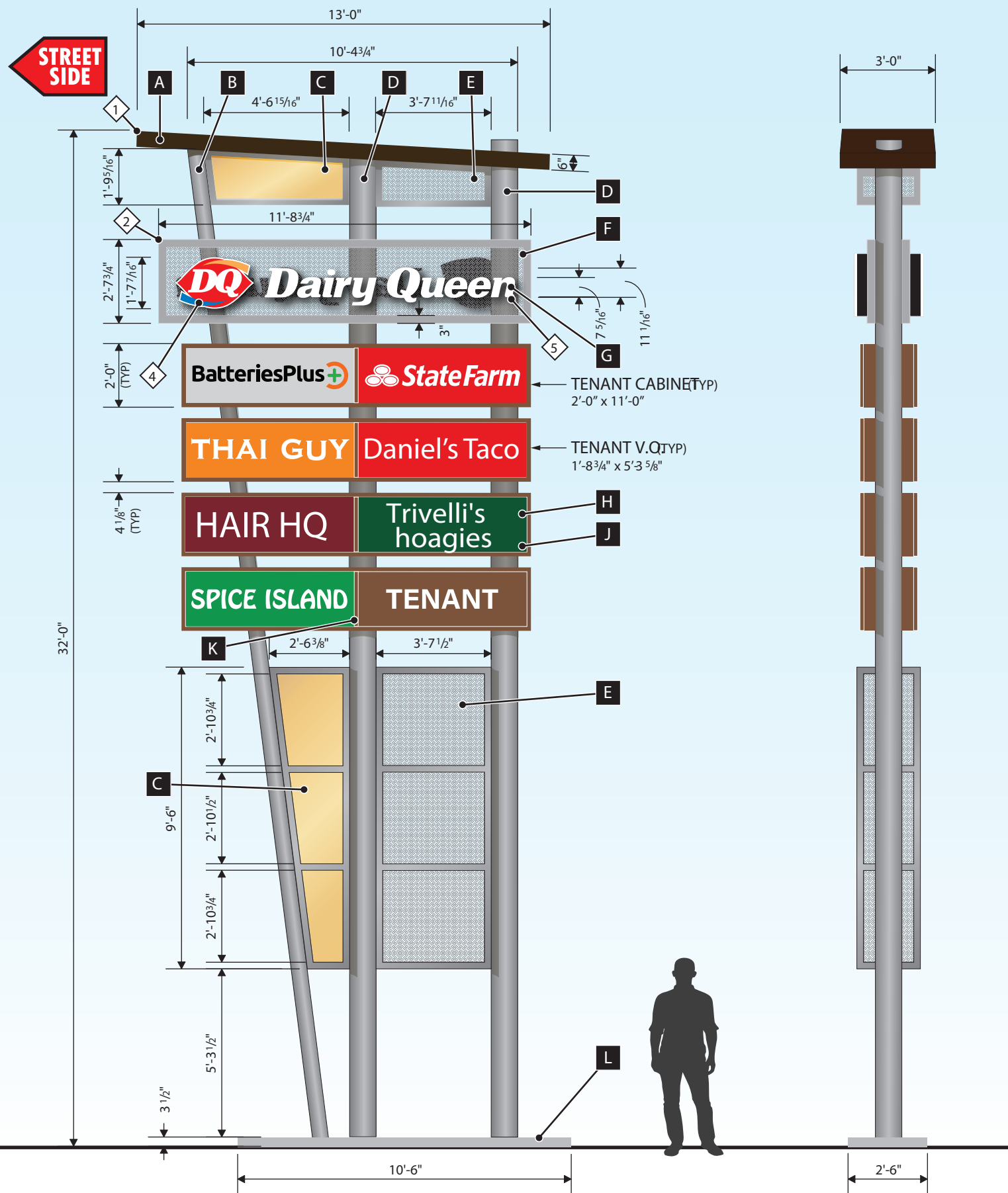
1 MULTI-TENANT PYLON - D/F, INTERNALLY ILLUMINATED: 3/8" = 1'-0" QUANTITY: 1 MANUFACTURE & INSTALL
