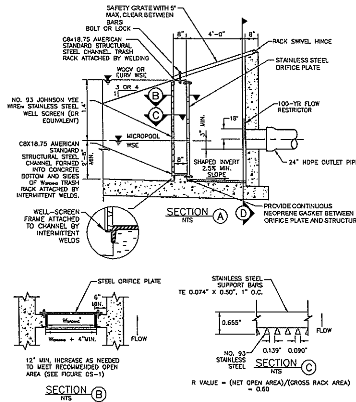
Figure OS-1. Trash Rack Sizing
