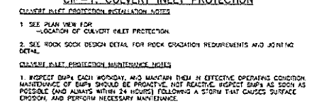
CIP-1. CULVERT INLET PROTECTION
