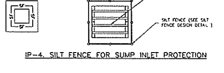
IP-4. SILT FENCE FOR SUMP INLET PROTECTION
