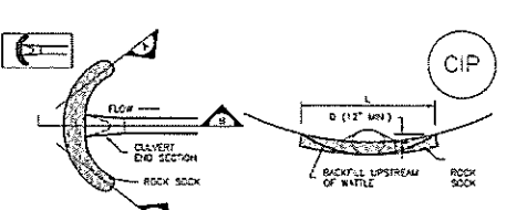
CIP-1. CULVERT INLET PROTECTION
