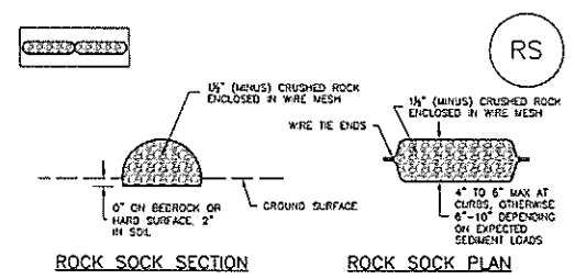
RS-1. ROCK SOCK PERIMETER CONTROL
