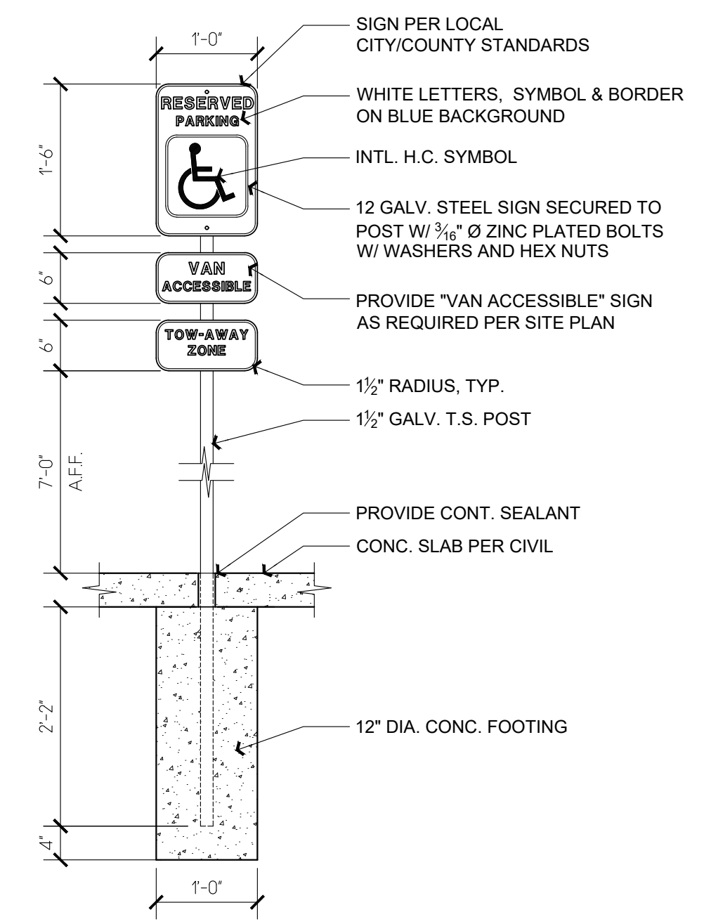
3 ACCESSIBLE SIGN SCALE: 3/4" = 1'-0"
